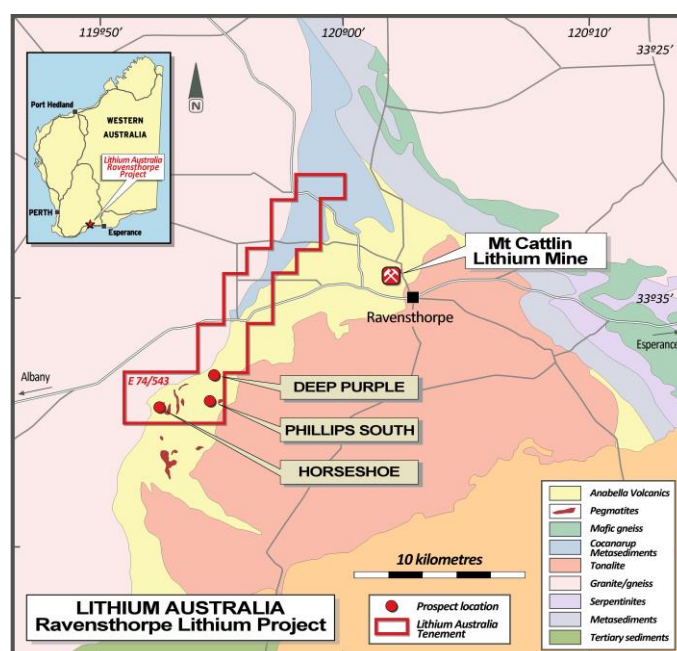
Figure 1 Regional geology of LIT's Ravensthorpe Project
