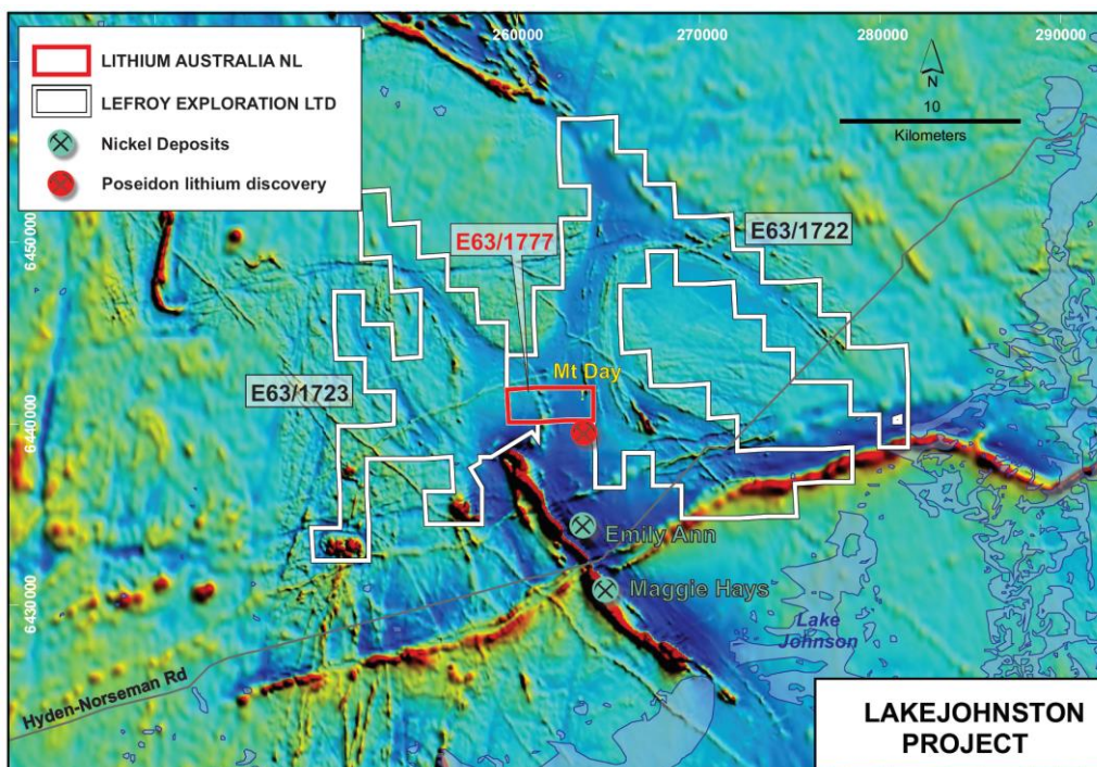
Figure 4: Consolidated project area comprising amalgamated lithium rights that benefit LIT. Brittle rocks, conducive to pegmatite intrusion, are represented by the darker blue hues in this magnetic image. The source magmas are probably preserved in the paler blue, ovoid structures.
